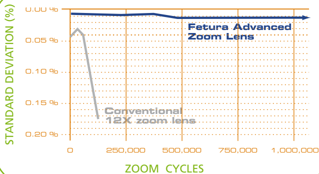
MAGNIFICATION REPEATABILITY *
